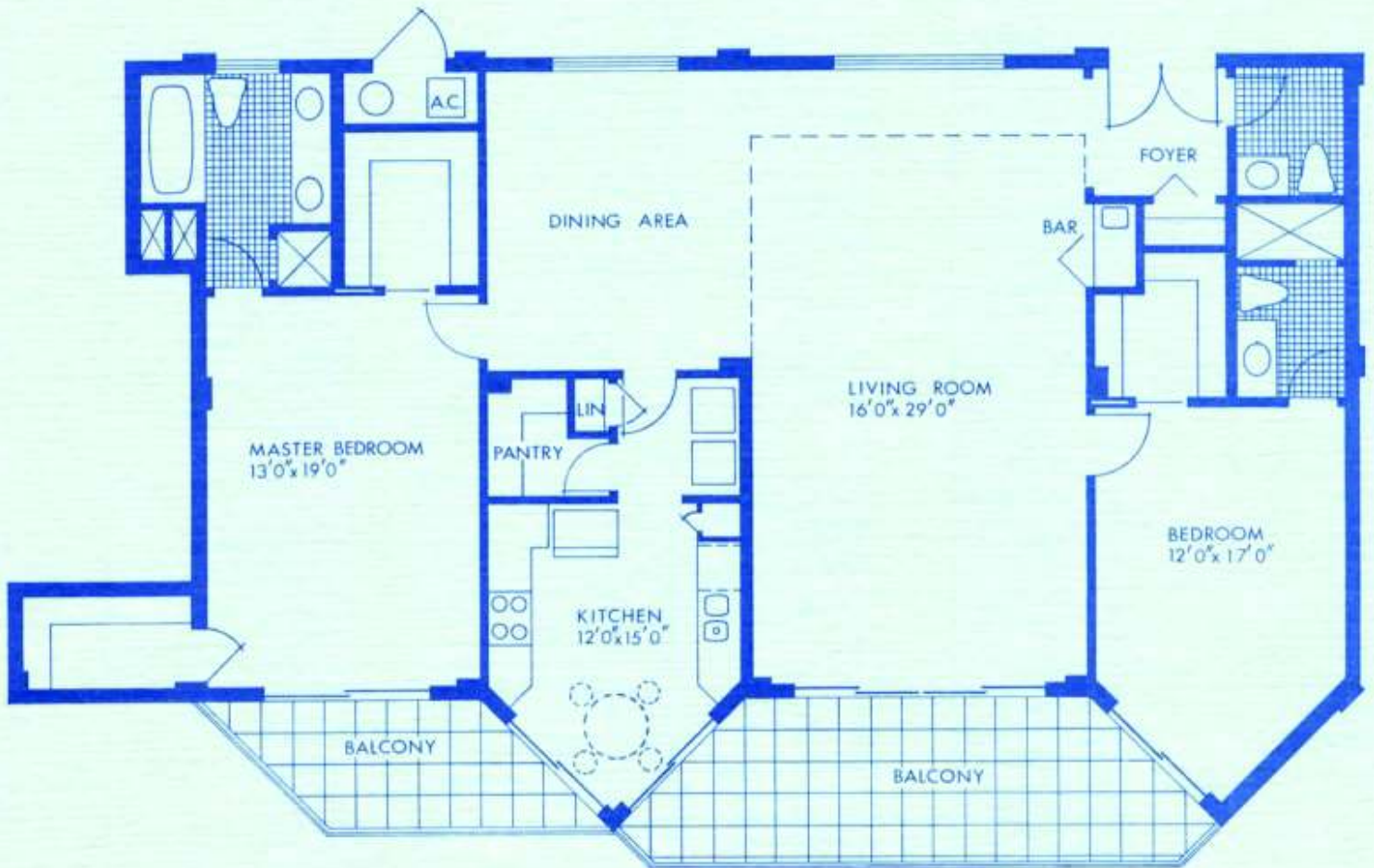
APARTMENT 05 FLOOR PLAN
